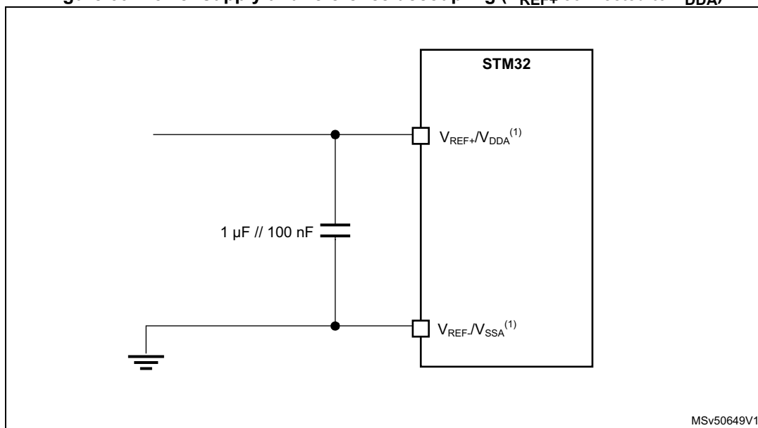
Figure 60. Power supply and reference decoupling ( V_{REF+} connected to V_{DDA} )
