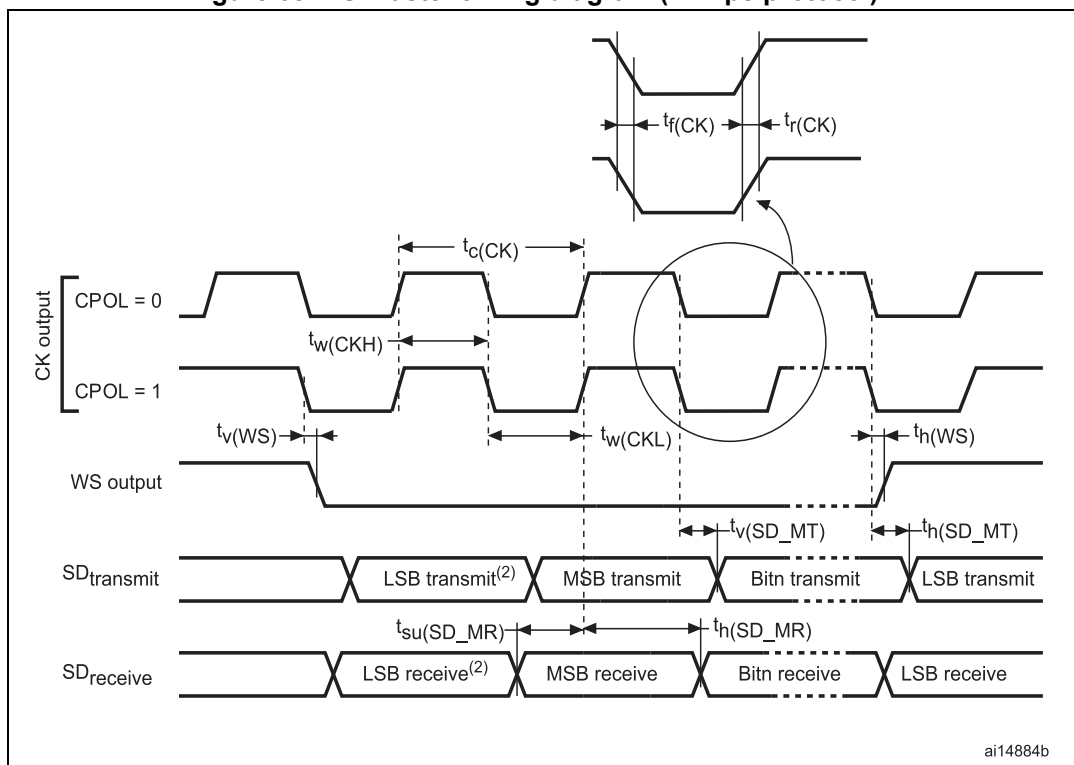
Figure 68. I 2 S master timing diagram (Philips protocol) (1)
