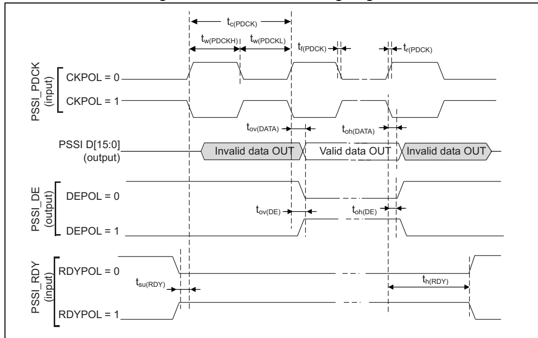
Figure 54. PSSI transmit timing diagram
